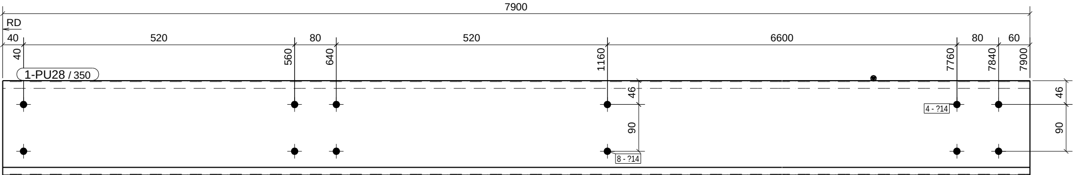
FRONT VIEW
